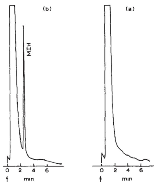
Fig. 3. Chromatograms of processed rat blood, (a) collected before exposing the rat to MIC and (b) collected after exposing the rat to a 3 LC_{50} dose of MIC for 30 min. In both instances 1 ml of blood was taken for processing and the final residue was diluted to 100 \mu l with ethyl acetate. Experimental conditions as in Fig. 2.
