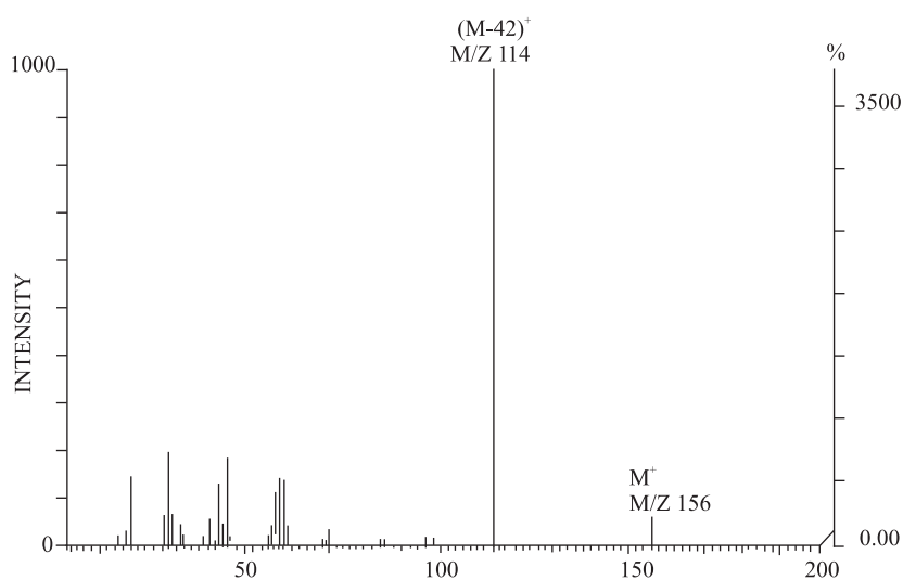
Figure 2. Mass Spectra of MIH (Standard)
