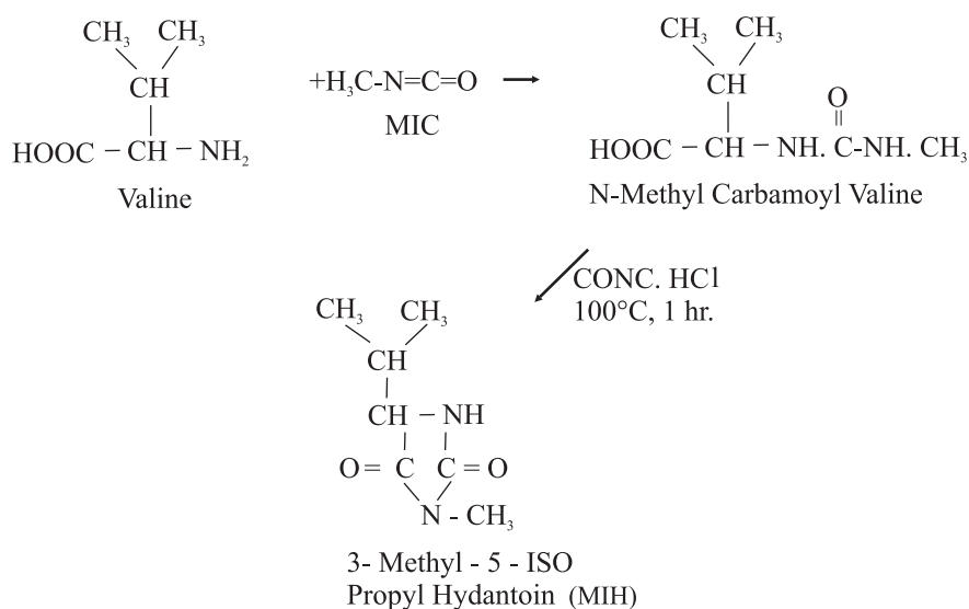
Figure 1. Reaction Sequence for MIH formation
