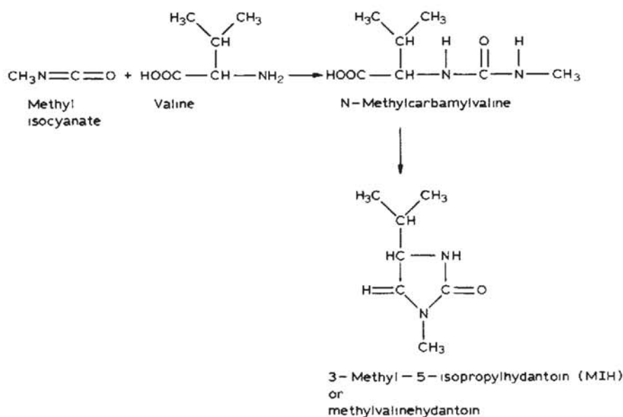
Fig 1. Reaction mechanism of haemoglobin carbamylation.
