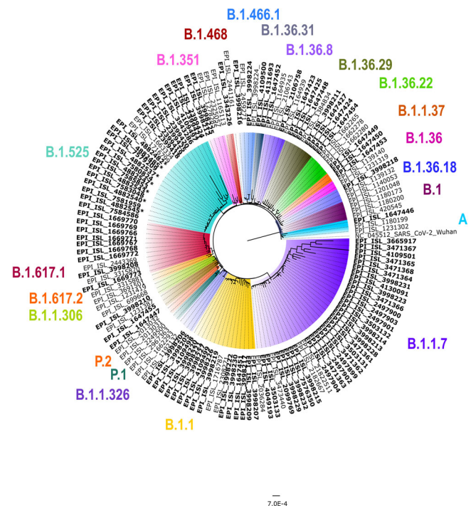
FIGURE 1 A neighbor-joining tree of the sequences retrieved from SARS-CoV-2 positive clinical samples and clinical isolates of the international travelers and local residents of India: A neighbor-joining tree was generated using a Tamura 3-parameter model with gamma distribution and a bootstrap replication of 1000 cycles. The sequences retrieved in this study are marked in black boldfaced. The alpha variant and Eta variant are marked with blue and orange color respectively
